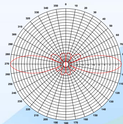
Radiation Pattern
